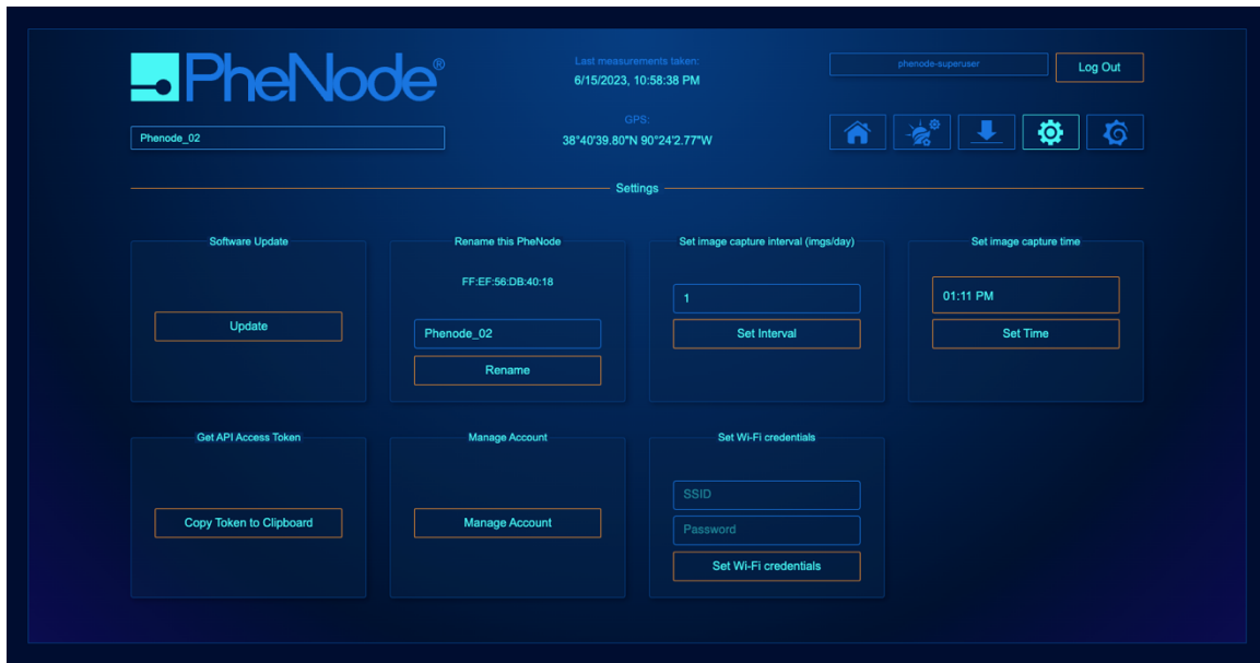
Figure 25. Settings Screen
