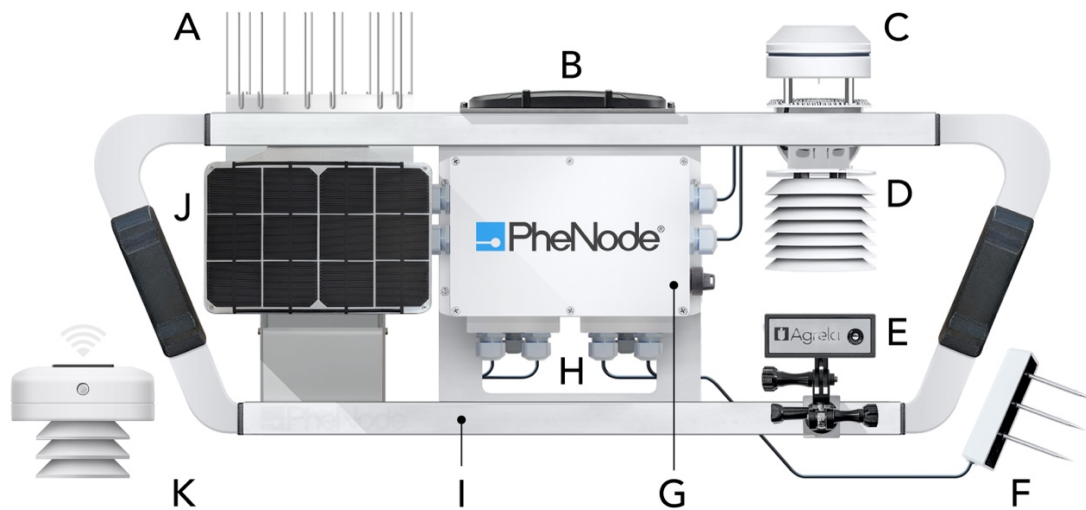
Figure 3. PheNode elements
